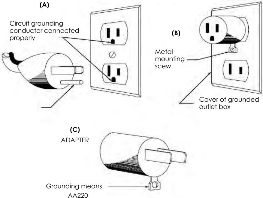
FIGURE 73.1 Grounding Methods
